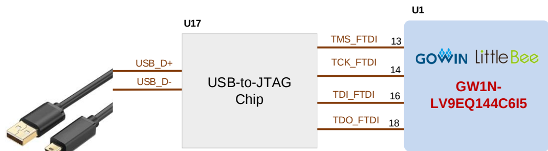
Figure 3-1 FPGA USB Download Diagram
