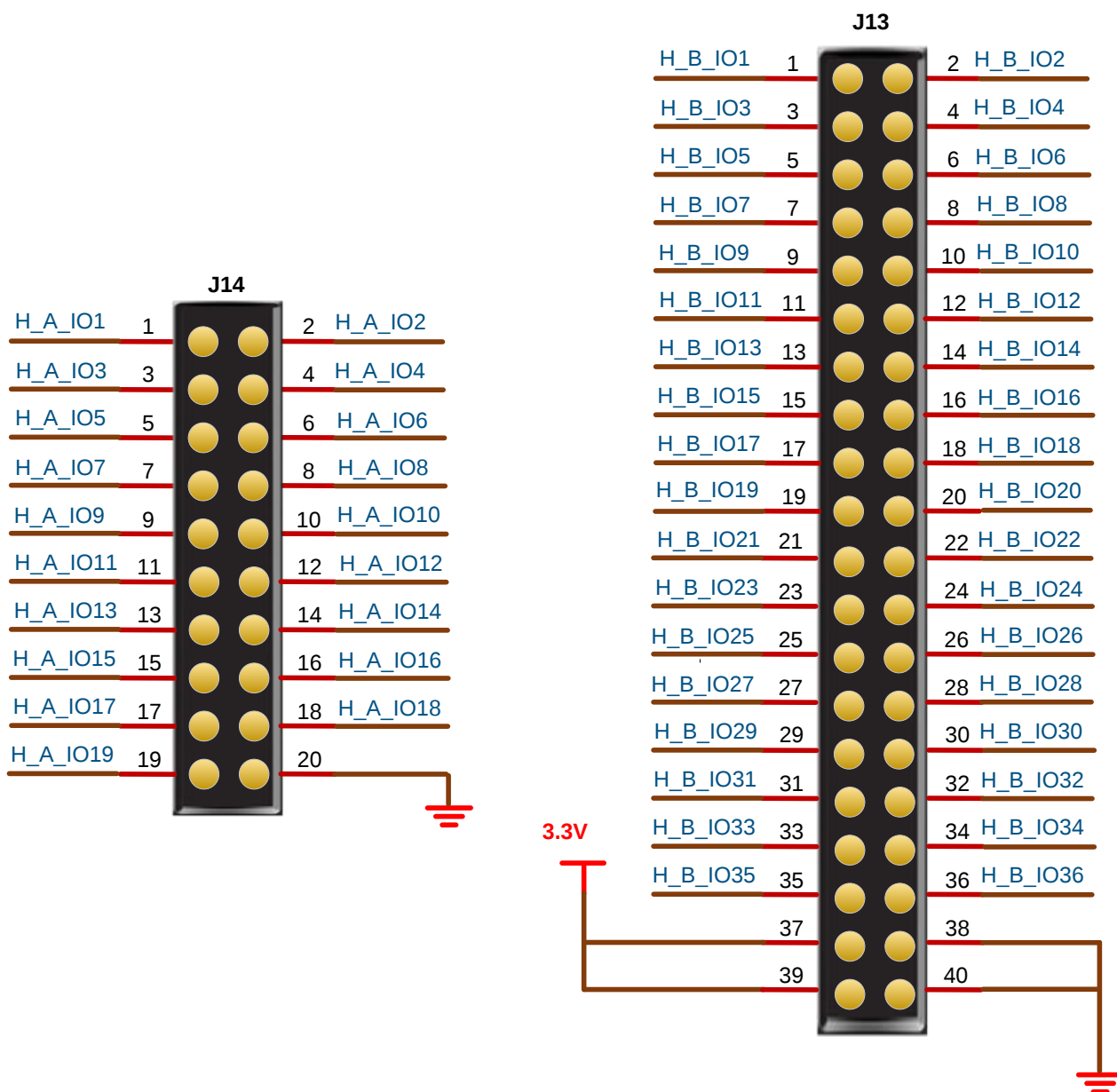
Figure 3-7 GPIO Circuit
