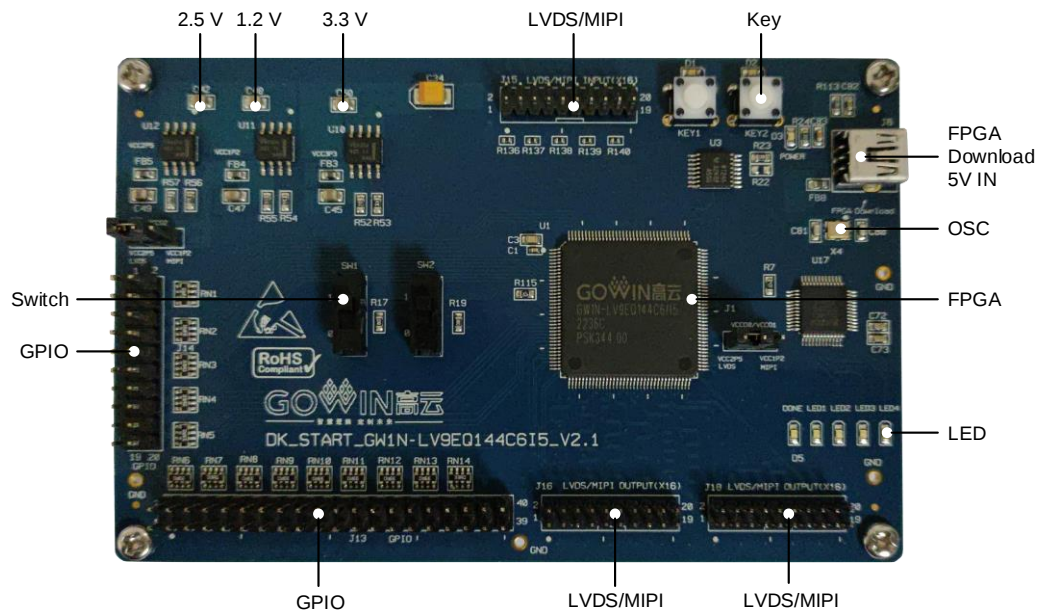
Figure 2-3 PCB Components
