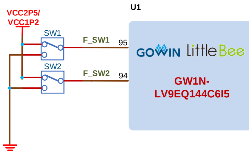
Figure 3-5 Switch Circuit
