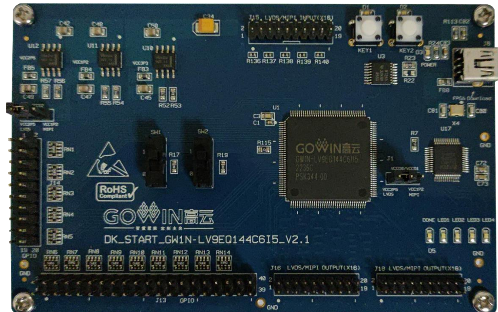
Figure 2-1 DK_START_GW1N-LV9EQ144C6I5_V2.1 Development Board
