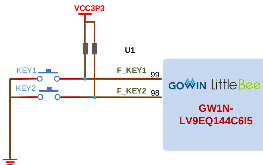
Figure 3-6 Key Circuit Diagram
