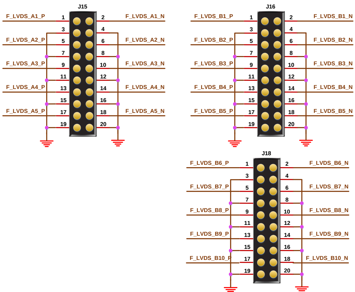
Figure 3-8 MIPI/LVDS Circuit
