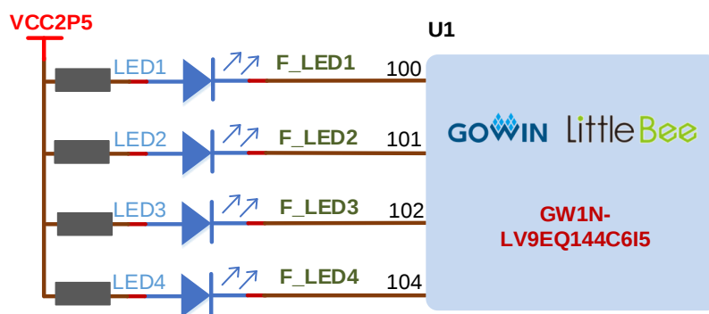
Figure 3-4 LED Circuit
